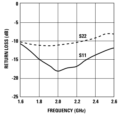
Figure 32. Input and Output Return Loss for 1900 MHz LNA.
