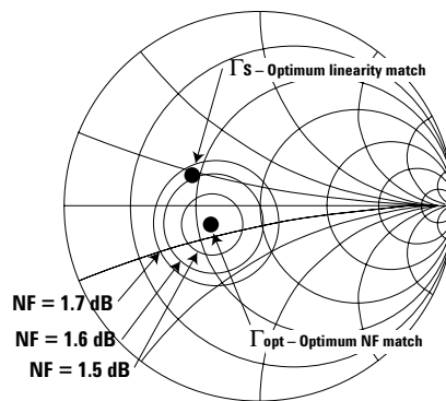
Figure 17. Noise figure performance.
