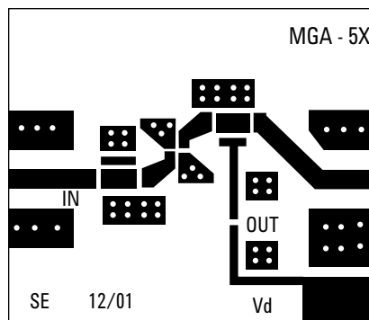
Figure 16. MGA-53453 PCB Layout.
