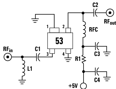
Figure 11. Schematic diagram with bias connections.
