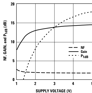
Figure 12. Gain, NF and P1dB vs. supply voltage at 1900 MHz.
