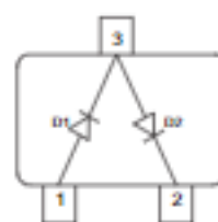
BAT64-04 BAT64-04W
