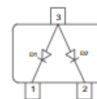
BAT64-06 BAT64-06W
