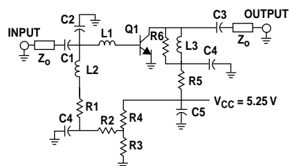
Figure 16. Schematic Diagram.
