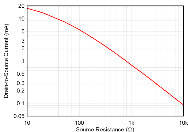
Figure 9-3. Drain-to-Source Current vs R_S , V_{DS} = 5 V
