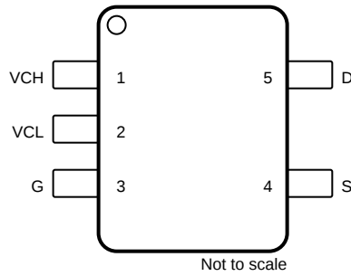
Figure 5-1. DBV (5-Pin SOT-23, Preview) and DCK (5-Pin SC70) Packages, Top View
