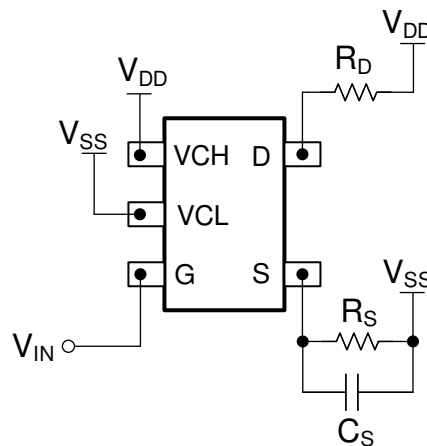
Figure 11-1. JFE150 Layout Example, Common Source Configuration
