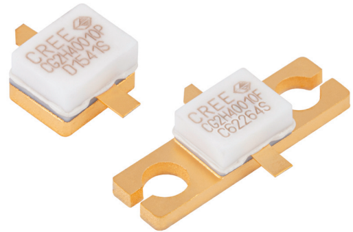
Package Types: 440196, & 440166 PNs: CG2H40010P & CG2H40010F
