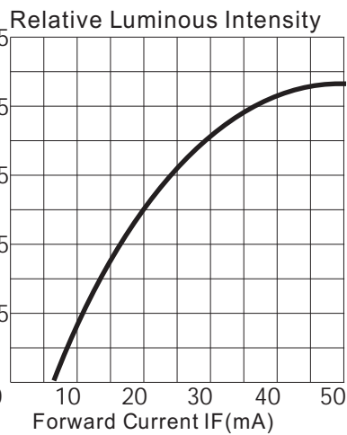
Relative Luminous Intensity VS. Forward Current
