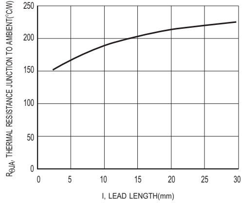
Figure2 Typical Thermal Resistance vs Lead Length
