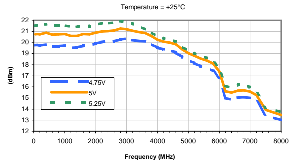
OUTPUT POWER at 1dB Compression vs. DEVICE VOLTAGE
