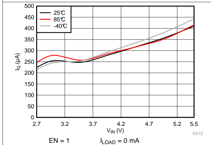
Figure 3. Quiescent Current
