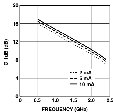
Figure 6. AT-31011 1 dB Compressed Gain vs. Frequency and Current at V_{\text{CE}} = 2.7\text{ V} .
