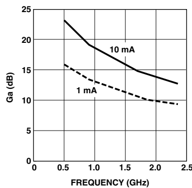
Figure 3. AT-31011 Associated Gain at Optimum Noise Match vs. Frequency and Current at V_{\text{CE}} = 2.7\text{ V} .
