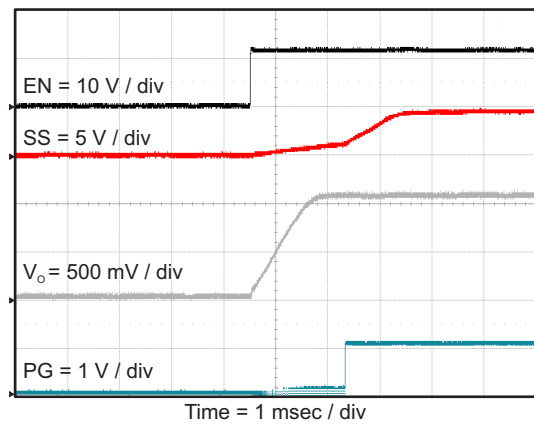
Figure 30. TPS562210 Start Up Relative To En
