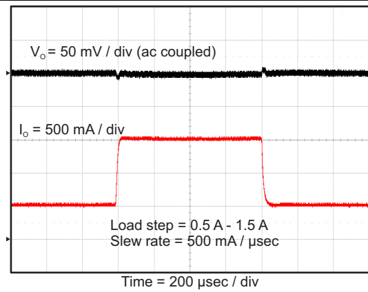
Figure 28. TPS562210 Transient Response
