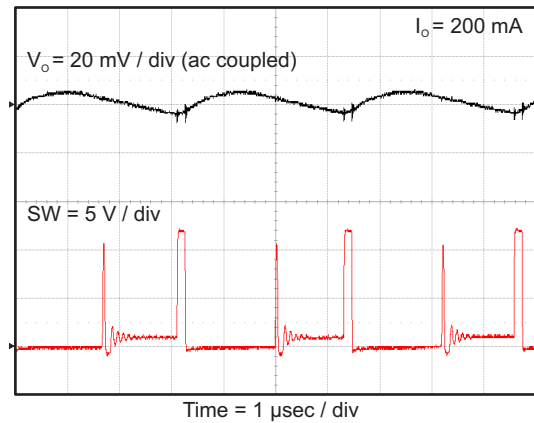
Figure 26. TPS562210 Output Voltage Ripple
