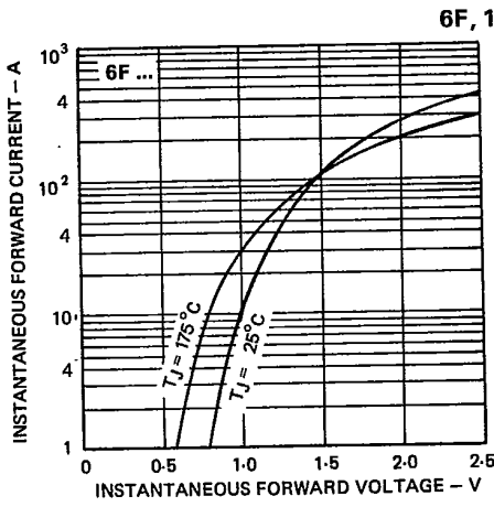
Fig. 5 - Maximum Forward Voltage Vs. Forward Current, 6F Series
