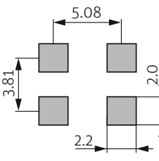
pad layout
