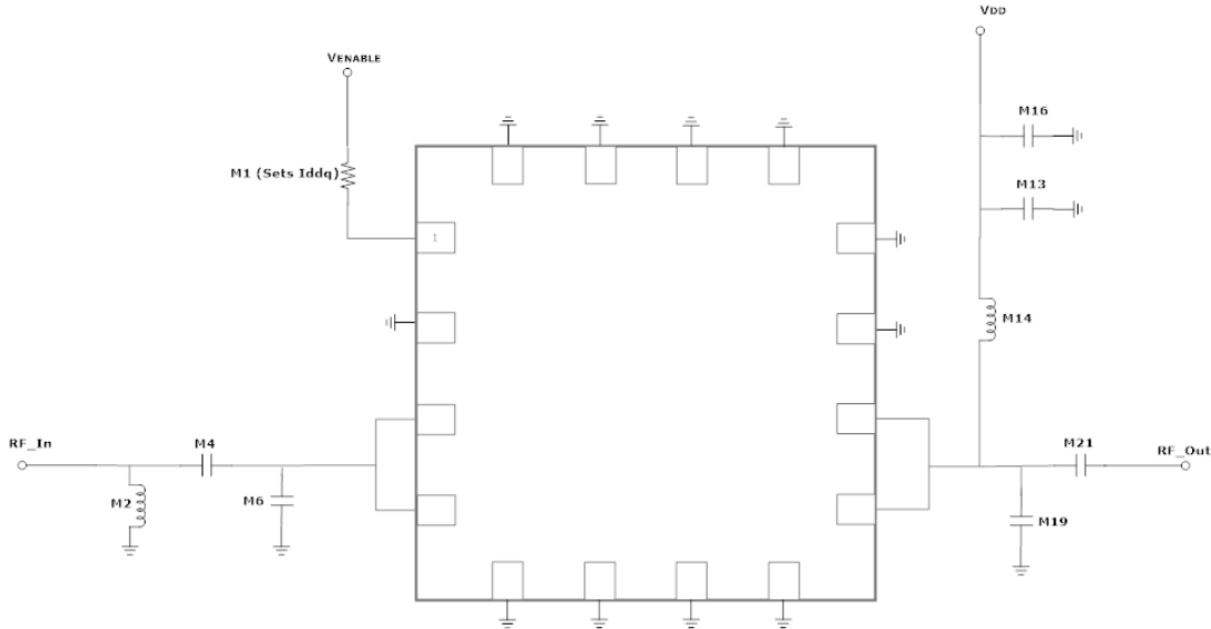
GRF5040 Application Schematic: (1.7 to 3.7 GHz)
