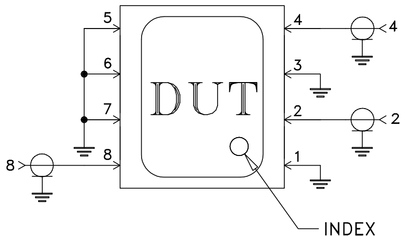
Schematic Diagram
