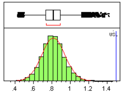
Figure 4. NF @ 10 GHz, Nominal=0.81, USL=1.50, CPK=1.8
